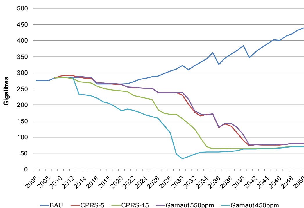
Figure 9.29: Water consumption by scenario, 2006-2050
