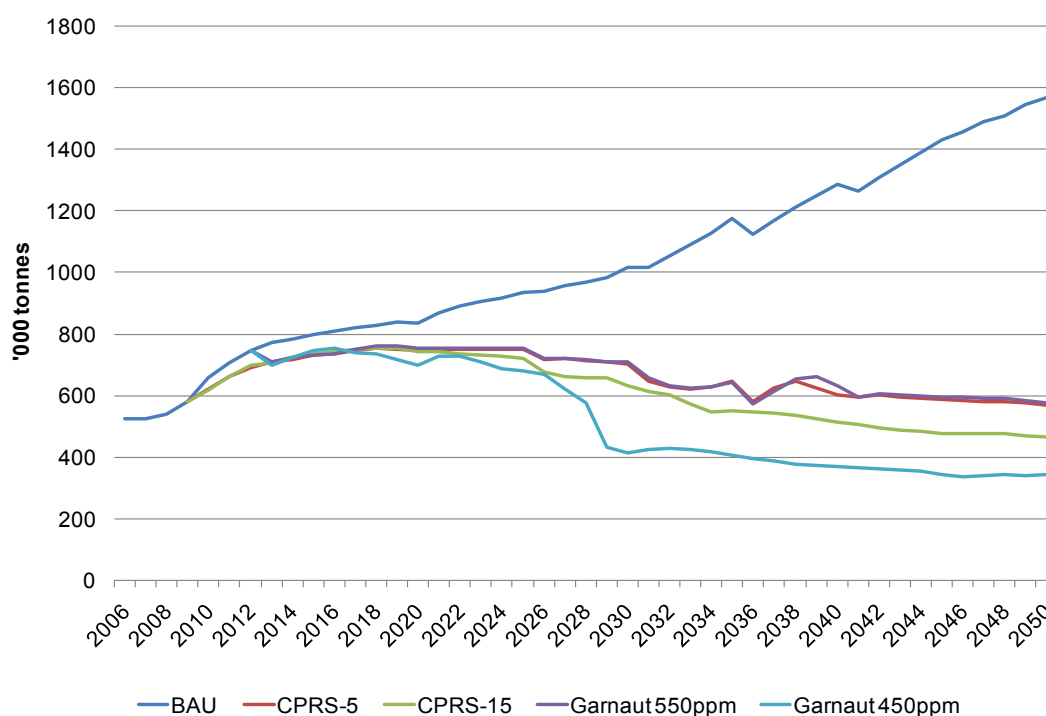
Figure 9.26: NO x emissions by scenario, 2006-2050
